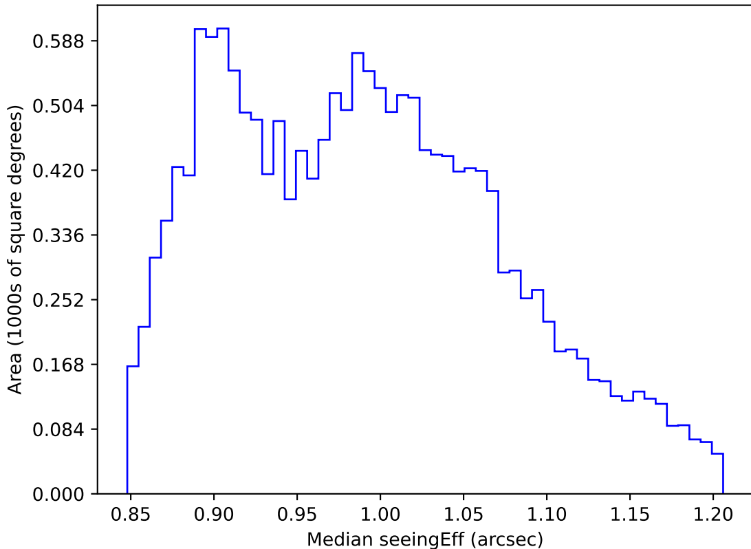
ddf_half_v3.4_10yrs WFD i band: Median seeingEff
