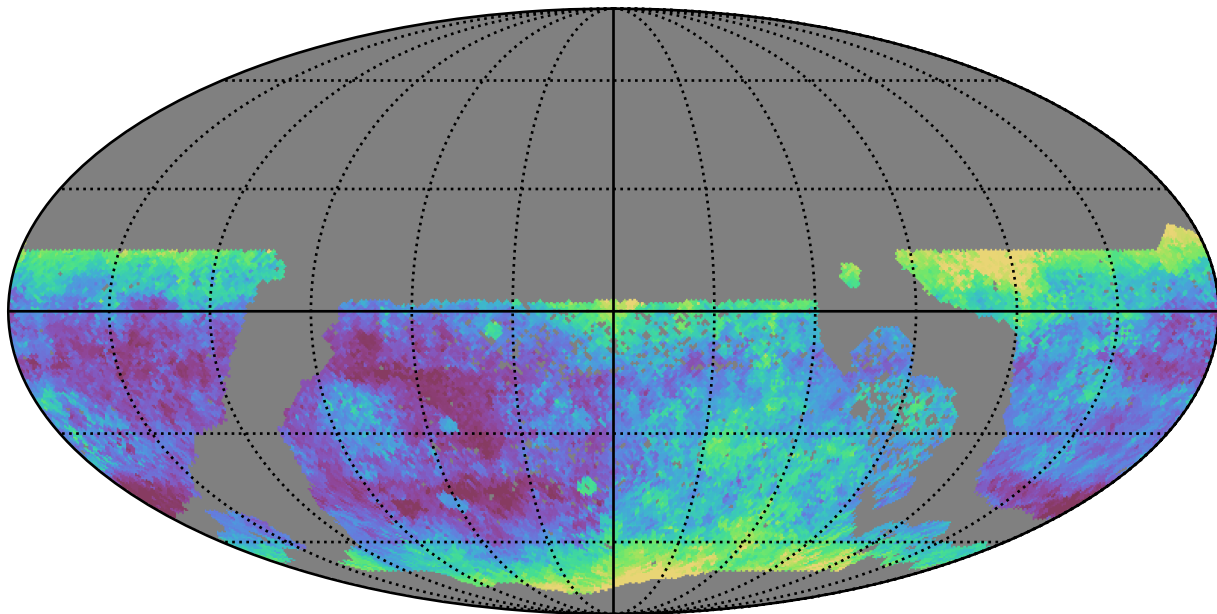
ddf_half_v3.4_10yrs WFD g band: Median seeingEff
