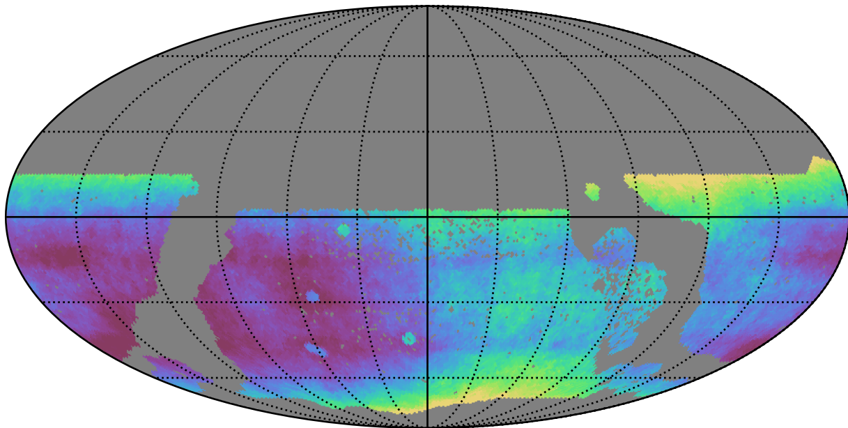
ddf_half_v3.4_10yrs WFD all bands: Median seeingEff
