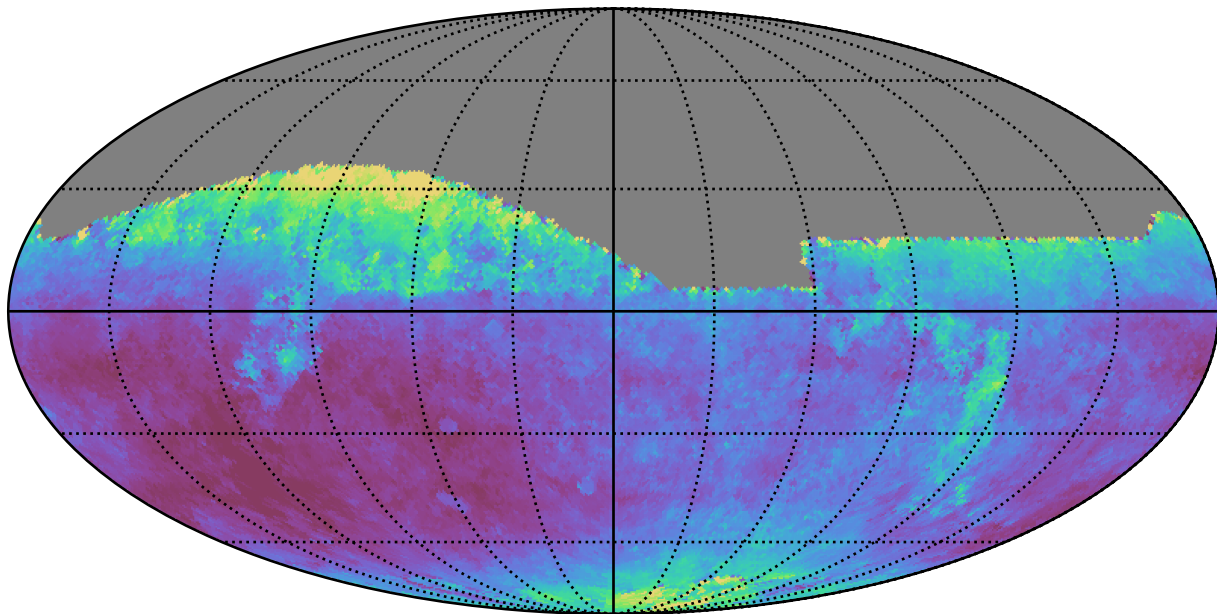
ddf_half_v3.4_10yrs All sky z band: Median seeingEff
