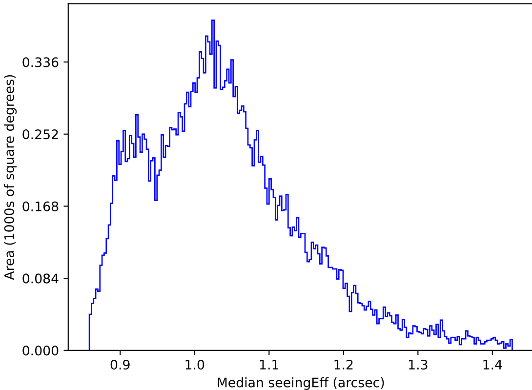
ddf_half_v3.4_10yrs All sky z band: Median seeingEff
