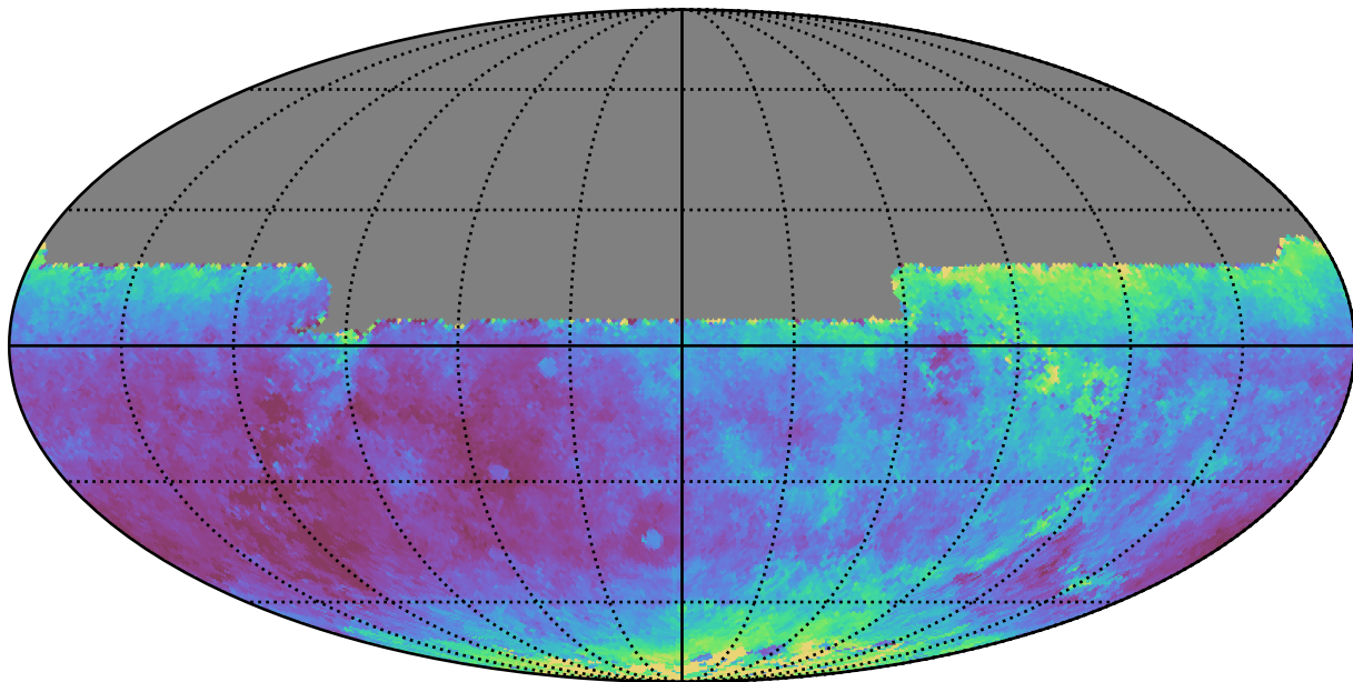
ddf_half_v3.4_10yrs All sky y band: Median seeingEff
