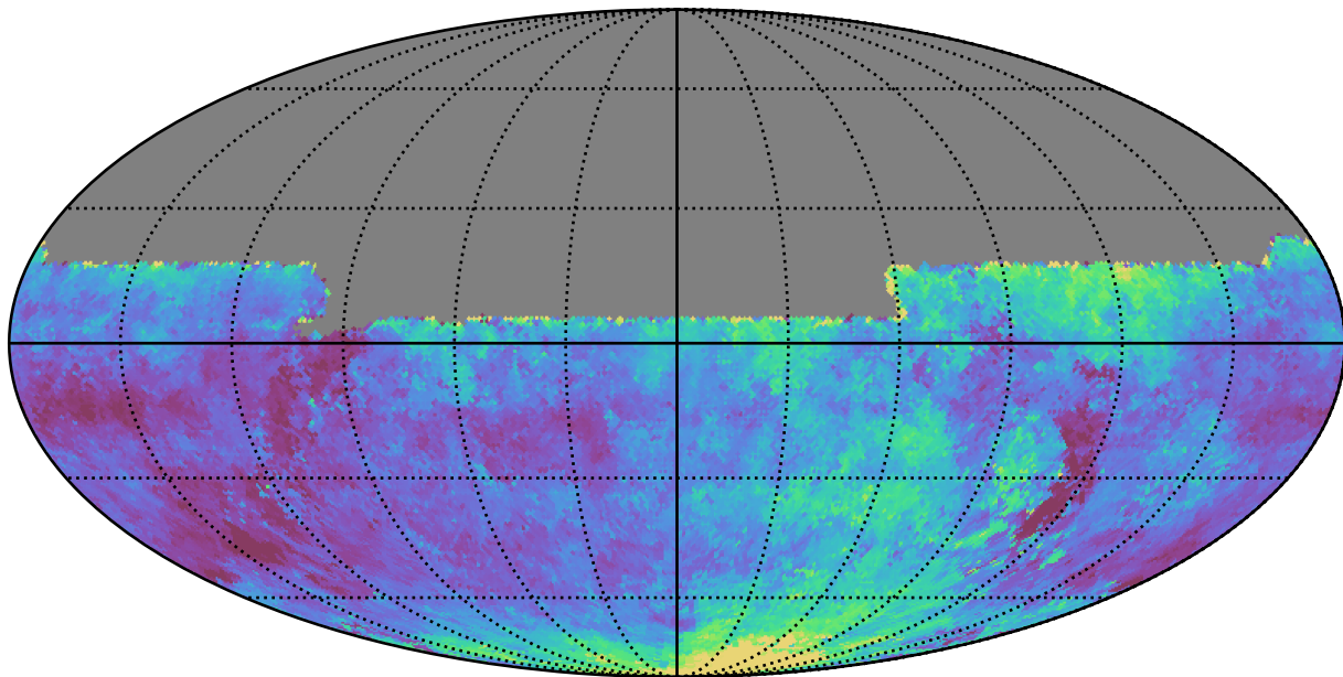
ddf_half_v3.4_10yrs All sky u band: Median seeingEff
