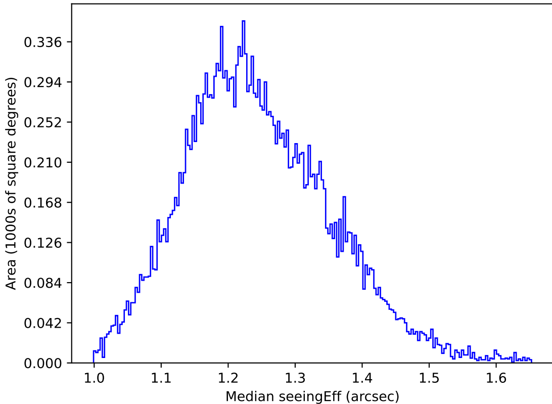
ddf_half_v3.4_10yrs All sky u band: Median seeingEff
