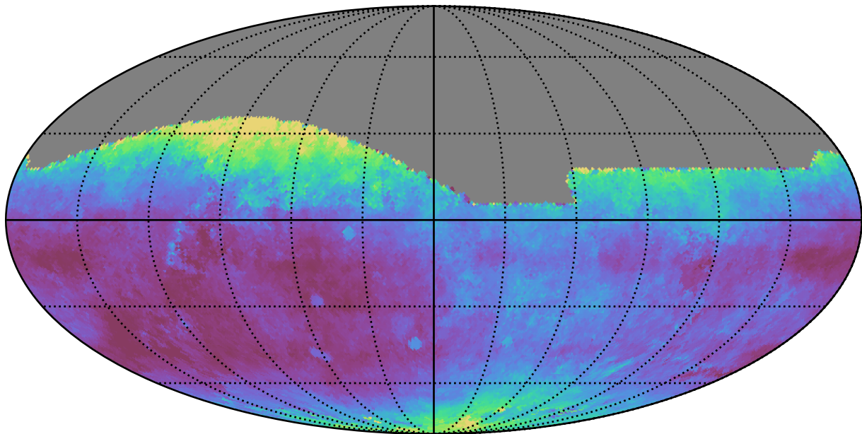
ddf_half_v3.4_10yrs All sky r band: Median seeingEff
