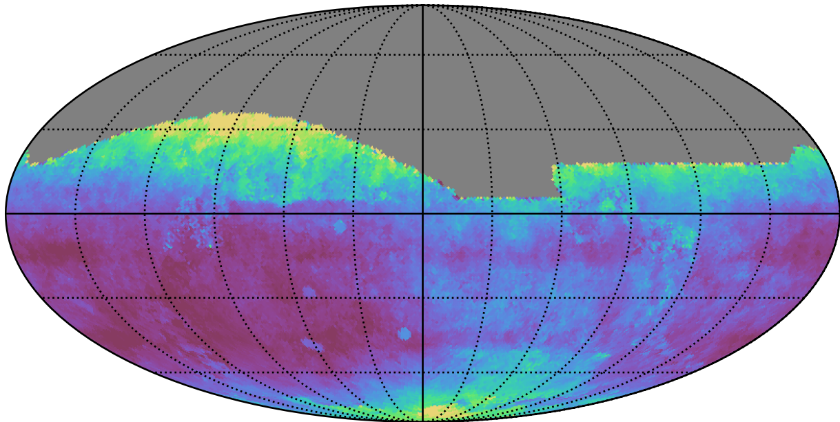
ddf_half_v3.4_10yrs All sky i band: Median seeingEff
