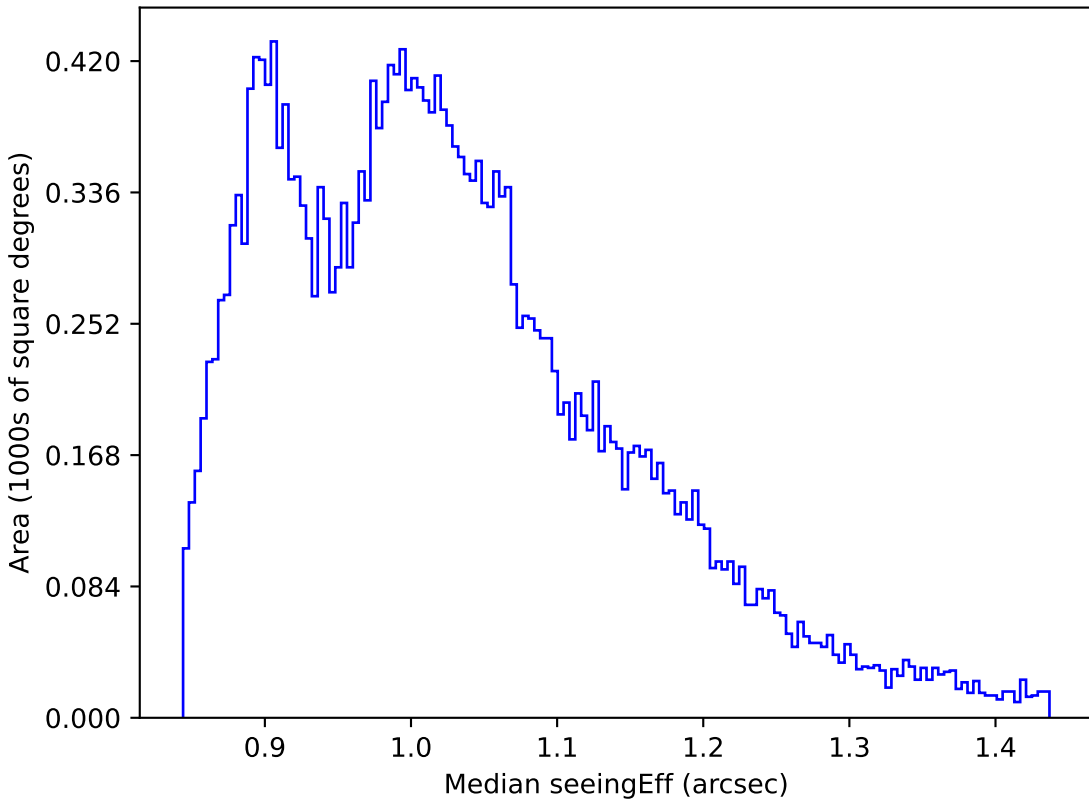
ddf_half_v3.4_10yrs All sky i band: Median seeingEff
