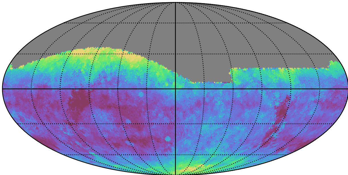
ddf_half_v3.4_10yrs All sky g band: Median seeingEff
