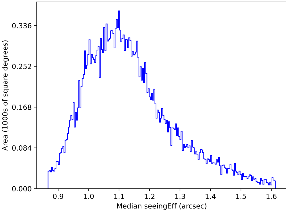
ddf_half_v3.4_10yrs All sky g band: Median seeingEff
