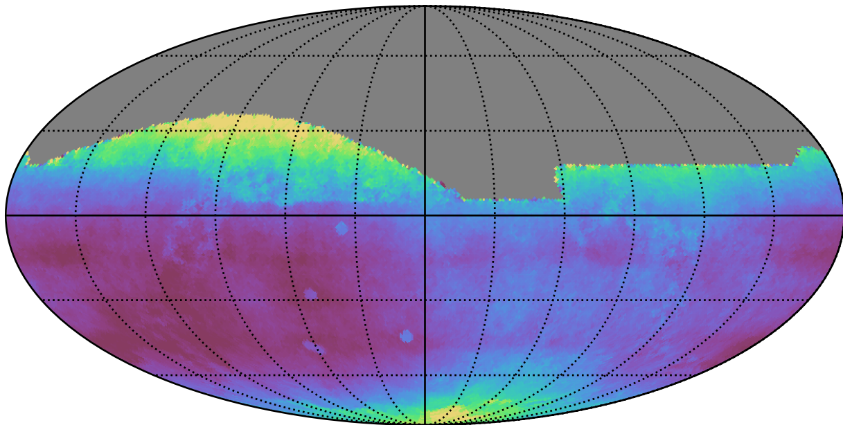
ddf_half_v3.4_10yrs All sky all bands: Median seeingEff
