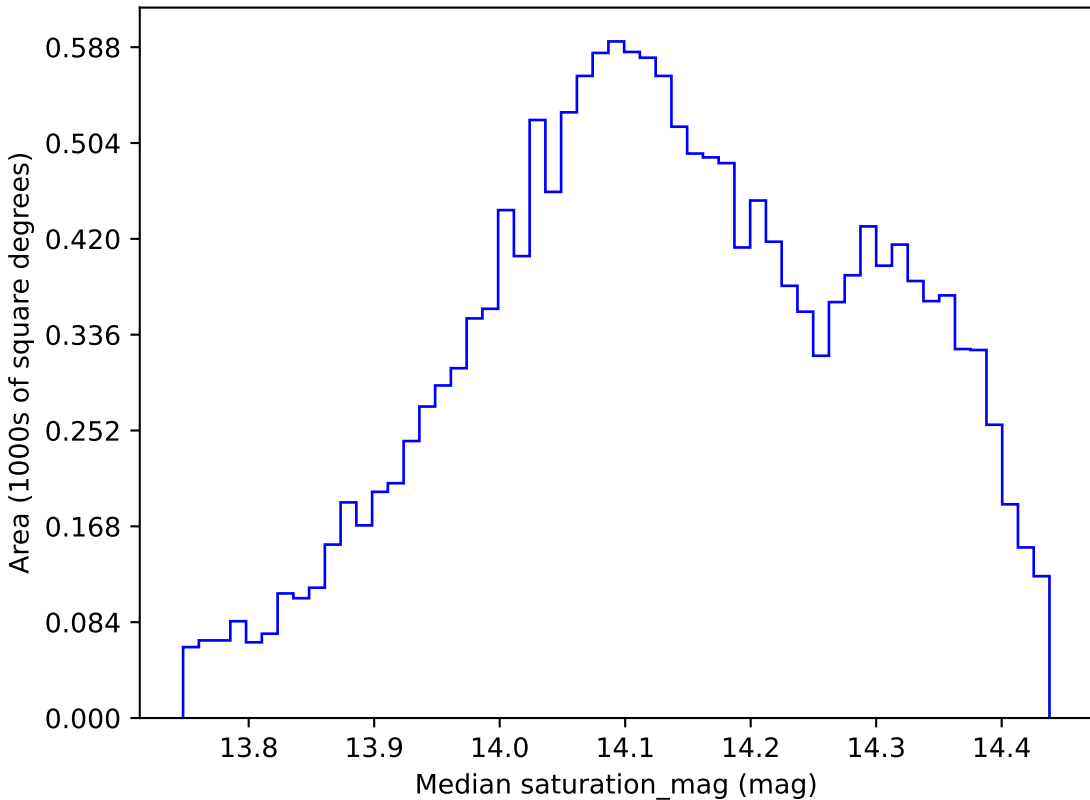
ddf_half_v3.4_10yrs WFD z band: Median saturation_mag
