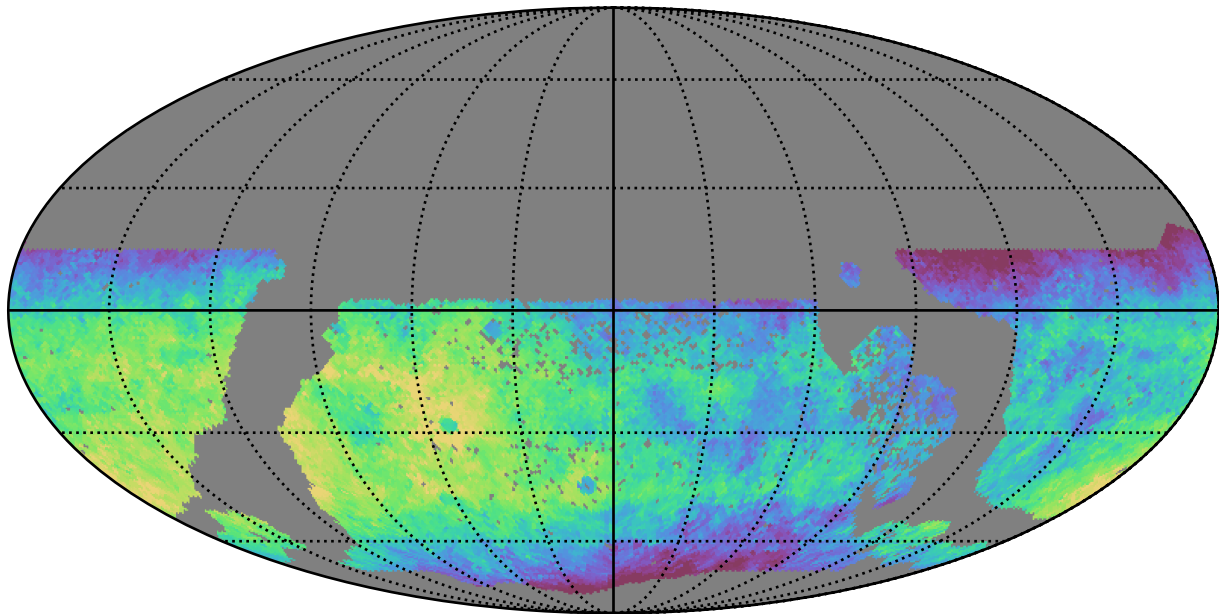
ddf_half_v3.4_10yrs WFD y band: Median saturation_mag
