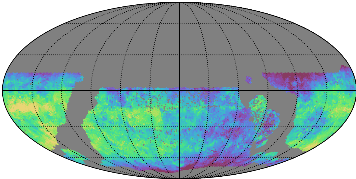
ddf_half_v3.4_10yrs WFD u band: Median saturation_mag
