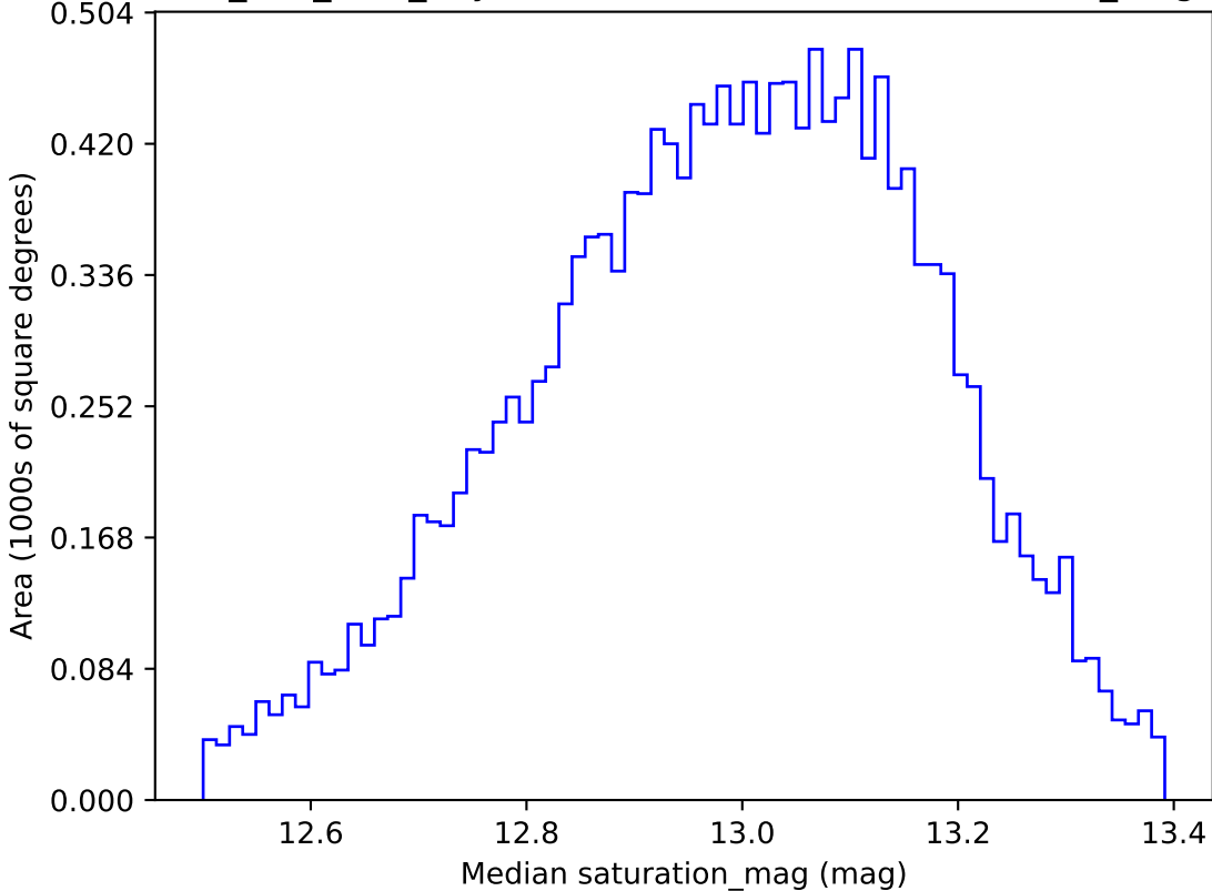
ddf_half_v3.4_10yrs WFD u band: Median saturation_mag
