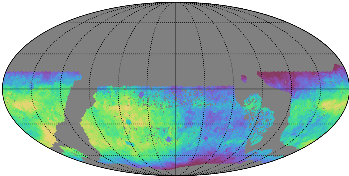
ddf_half_v3.4_10yrs WFD r band: Median saturation_mag
