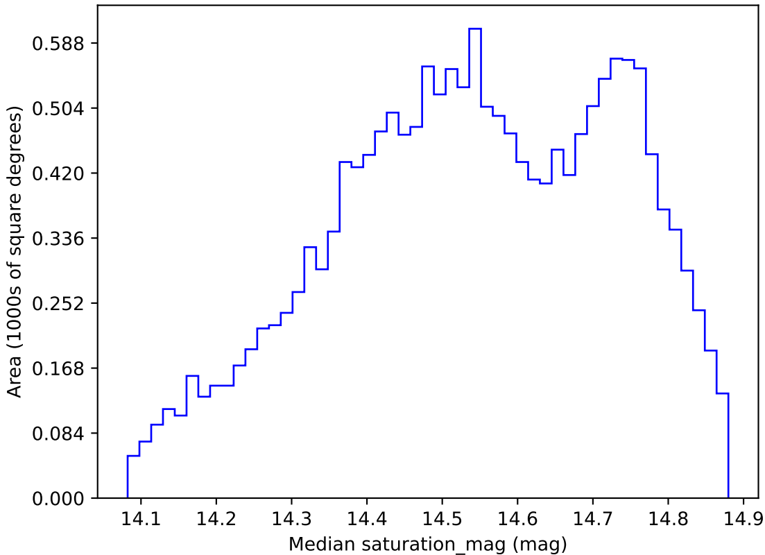
ddf_half_v3.4_10yrs WFD i band: Median saturation_mag
