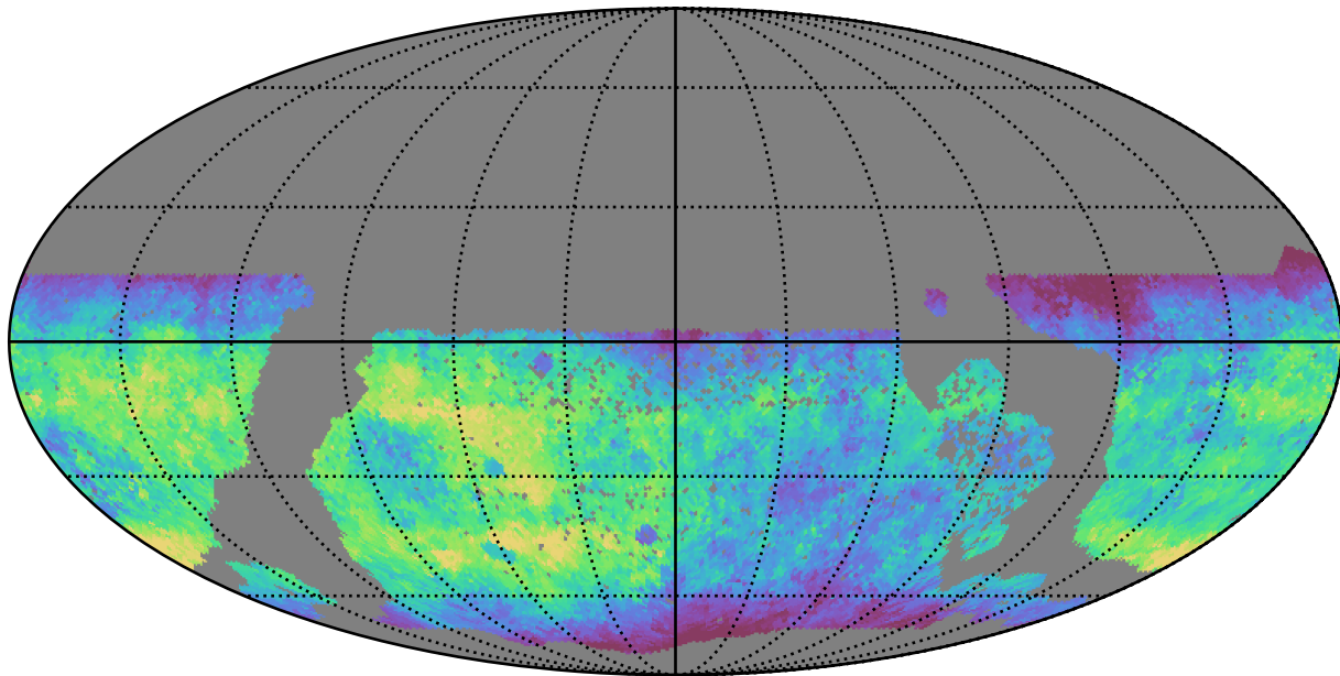
ddf_half_v3.4_10yrs WFD g band: Median saturation_mag
