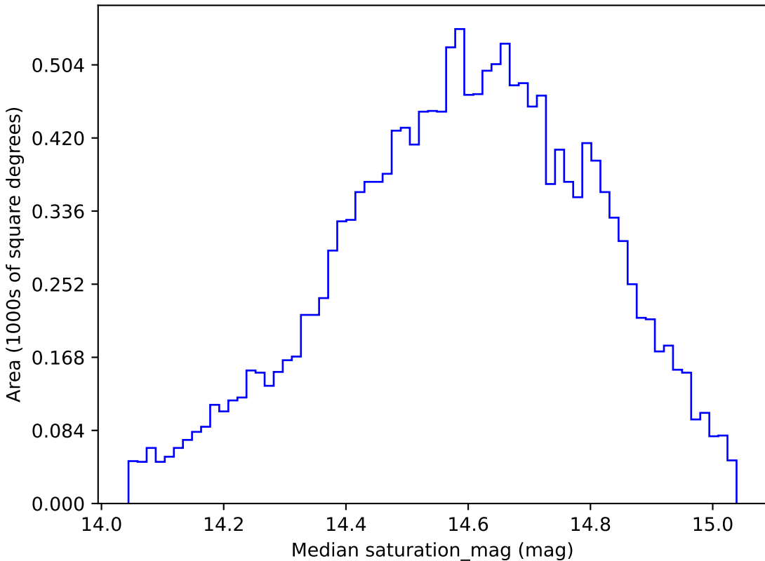
ddf_half_v3.4_10yrs WFD g band: Median saturation_mag
