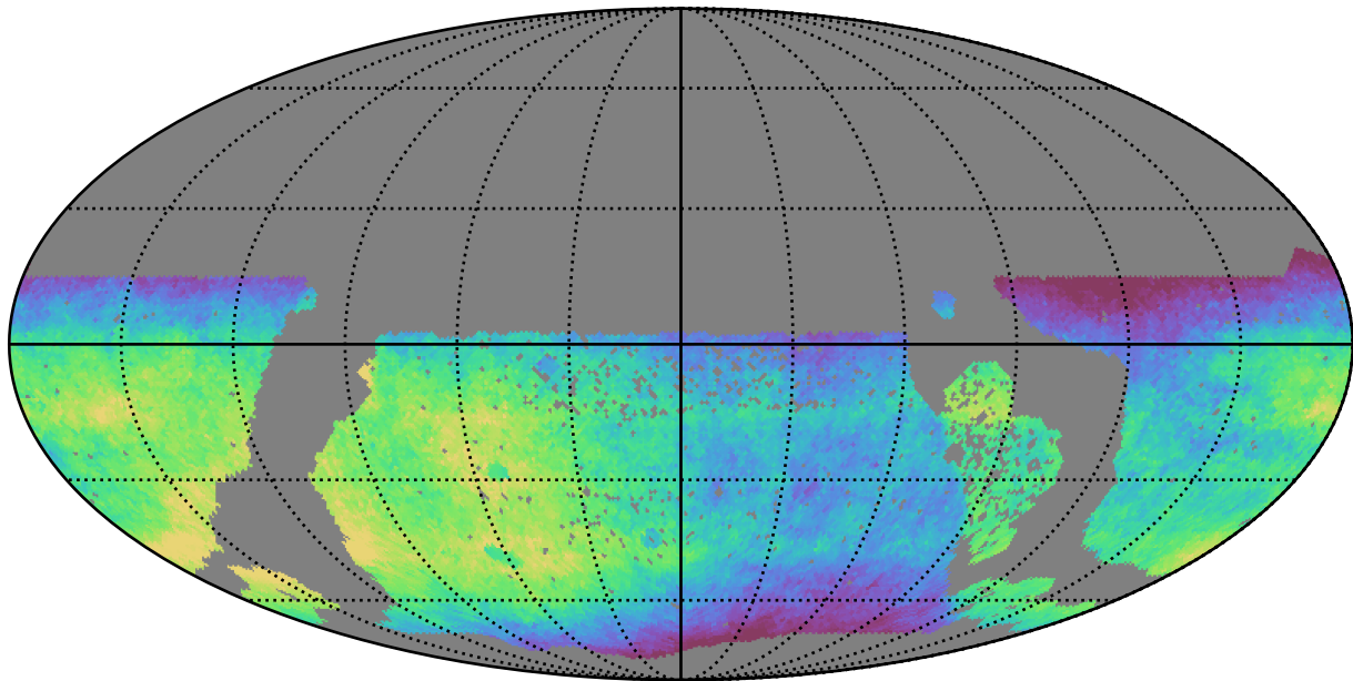
ddf_half_v3.4_10yrs WFD all bands: Median saturation_mag
