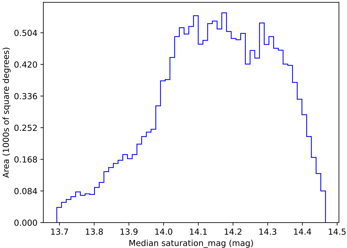
ddf_half_v3.4_10yrs WFD all bands: Median saturation_mag
