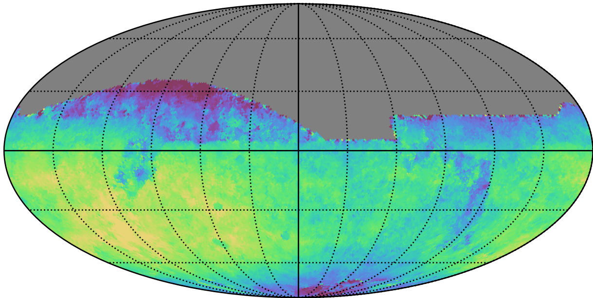
ddf_half_v3.4_10yrs All sky z band: Median saturation_mag
