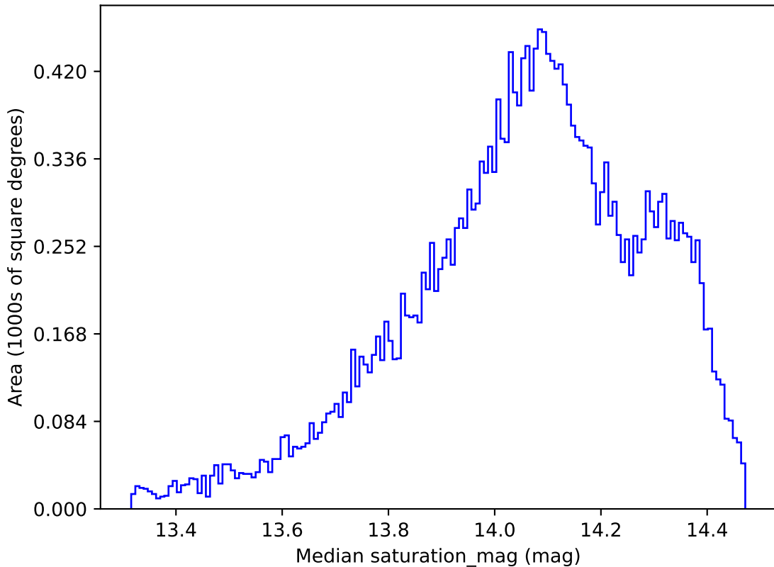
ddf_half_v3.4_10yrs All sky z band: Median saturation_mag
