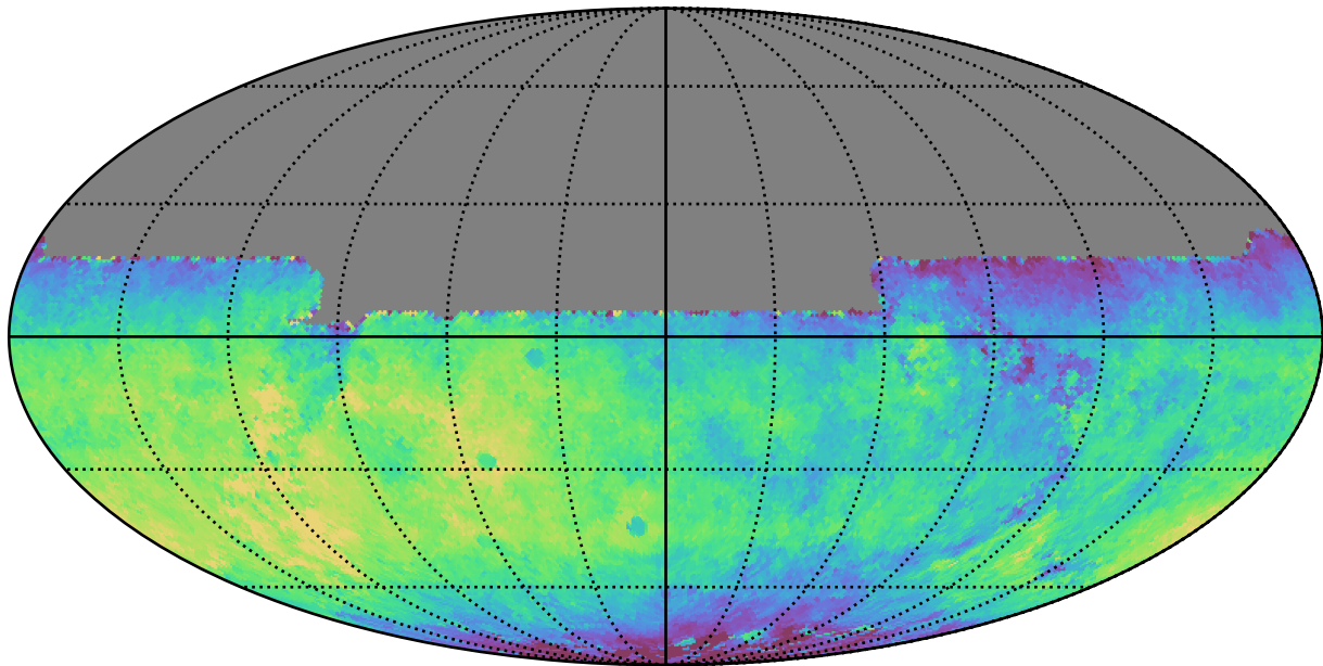
ddf_half_v3.4_10yrs All sky y band: Median saturation_mag
