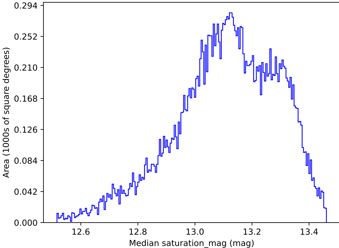
ddf_half_v3.4_10yrs All sky y band: Median saturation_mag
