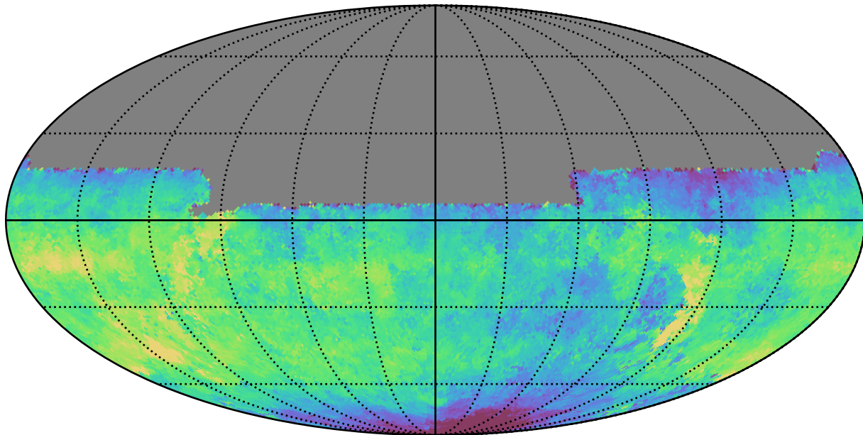
ddf_half_v3.4_10yrs All sky u band: Median saturation_mag
