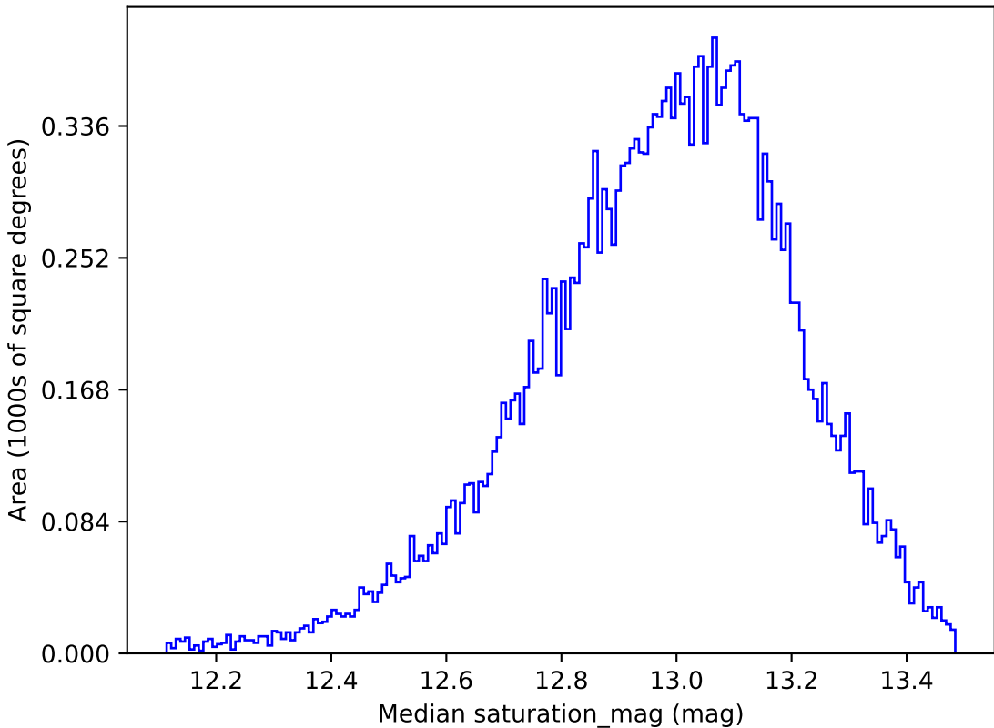
ddf_half_v3.4_10yrs All sky u band: Median saturation_mag
