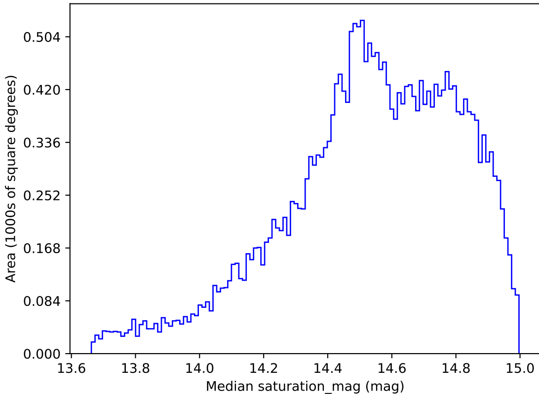
ddf_half_v3.4_10yrs All sky r band: Median saturation_mag
