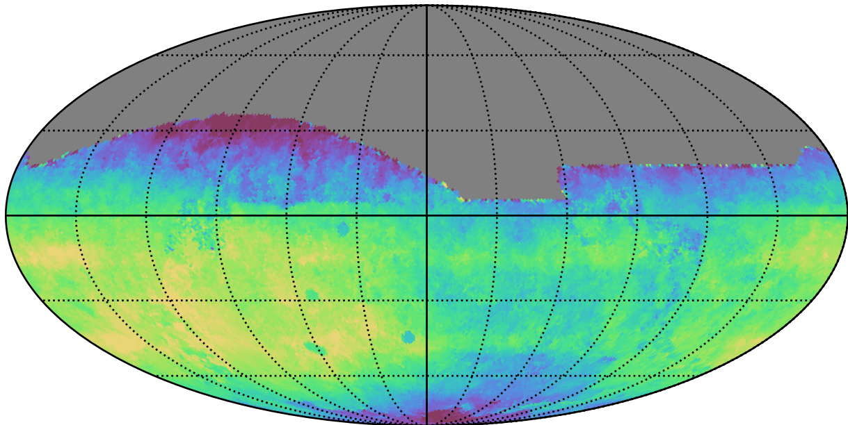
ddf_half_v3.4_10yrs All sky i band: Median saturation_mag
