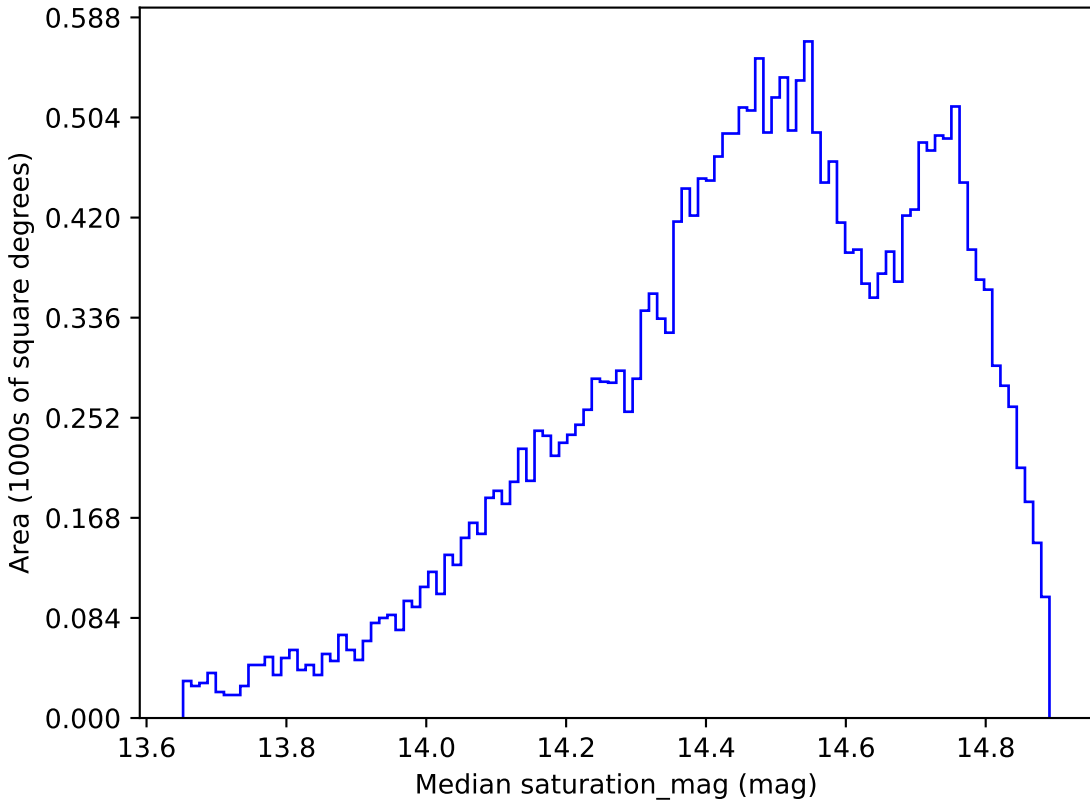
ddf_half_v3.4_10yrs All sky i band: Median saturation_mag
