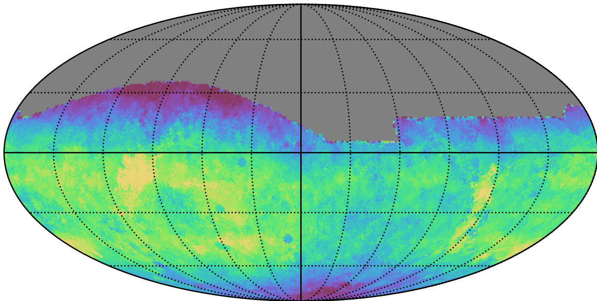
ddf_half_v3.4_10yrs All sky g band: Median saturation_mag
