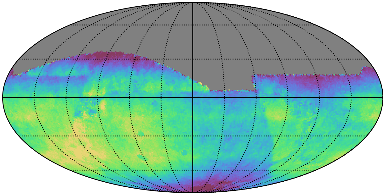
ddf_half_v3.4_10yrs All sky all bands: Median saturation_mag
