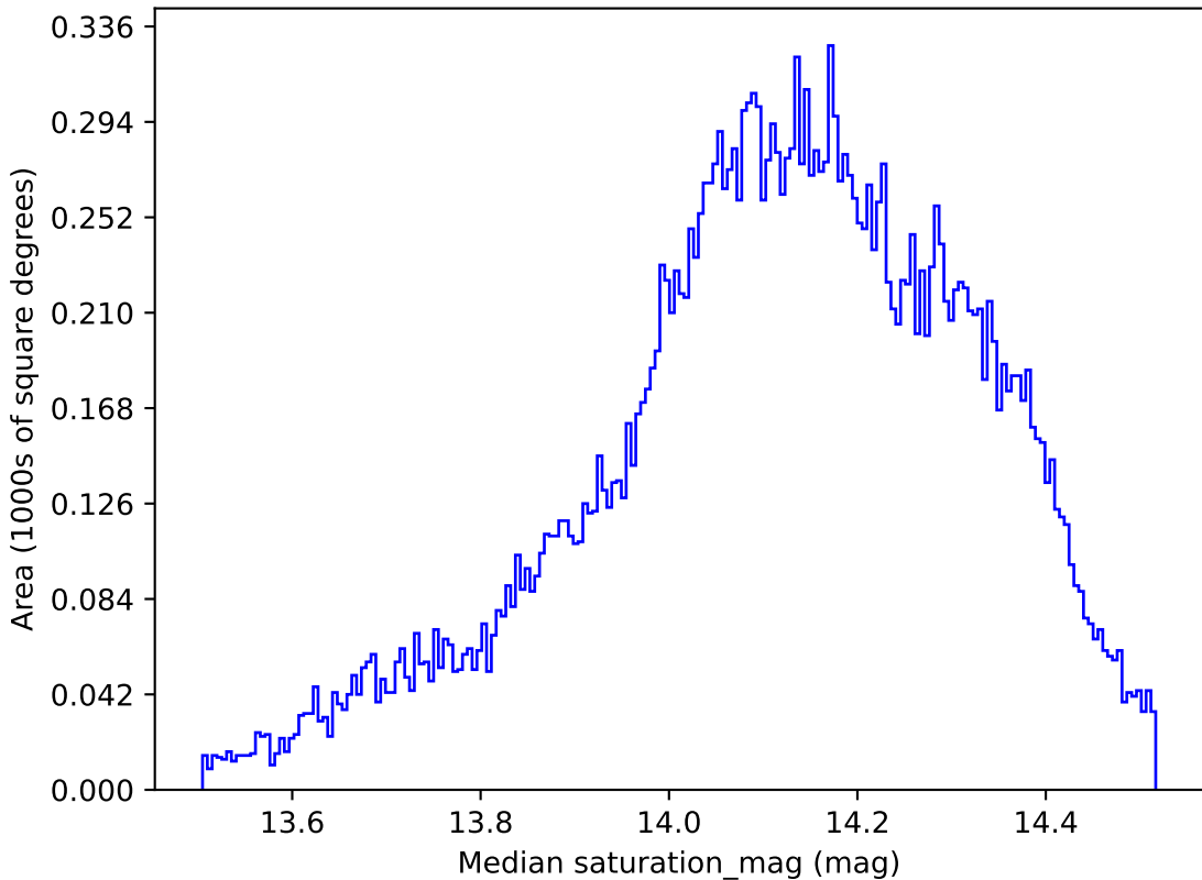
ddf_half_v3.4_10yrs All sky all bands: Median saturation_mag
