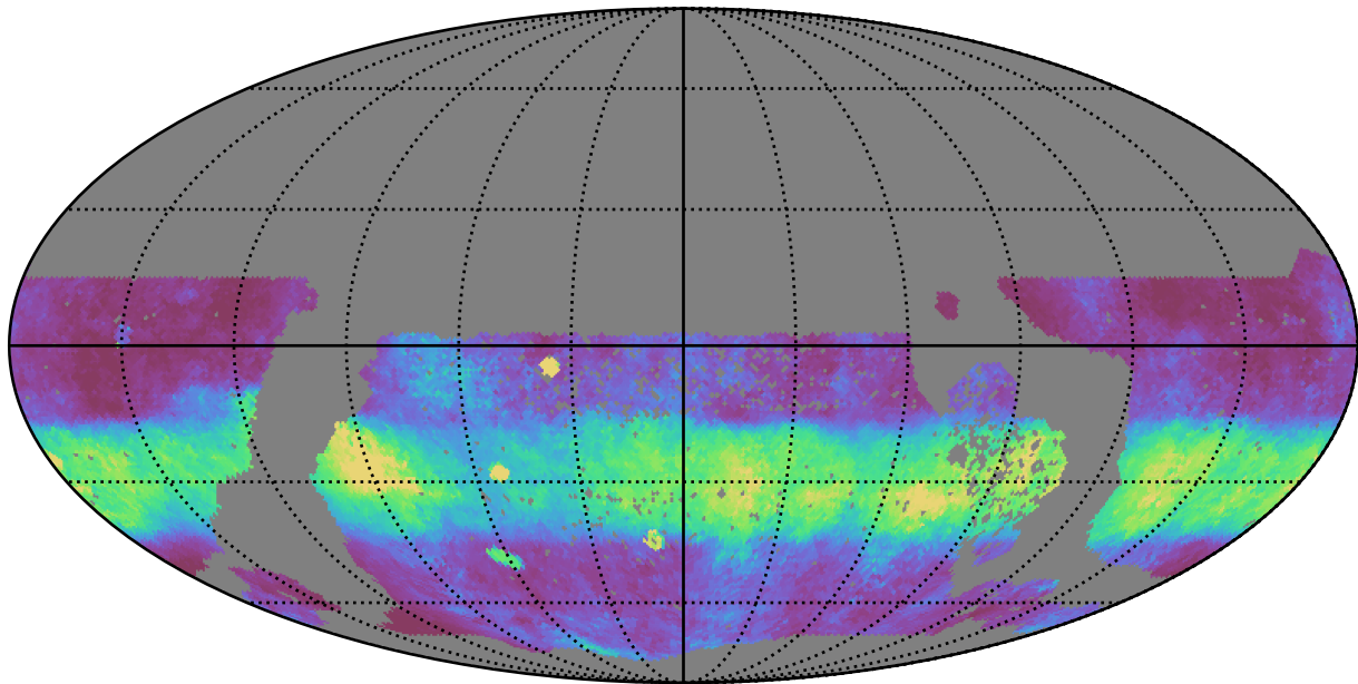
ddf_half_v3.4_10yrs WFD z band: Median normairmass
