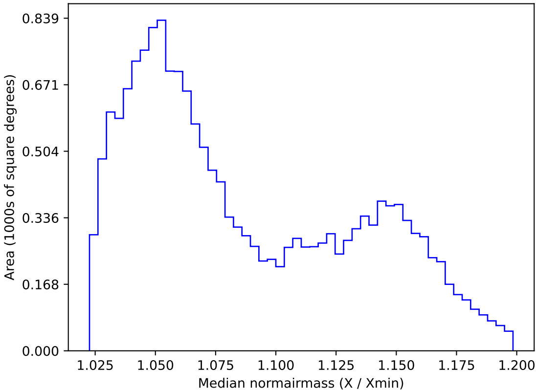
ddf_half_v3.4_10yrs WFD z band: Median normairmass
