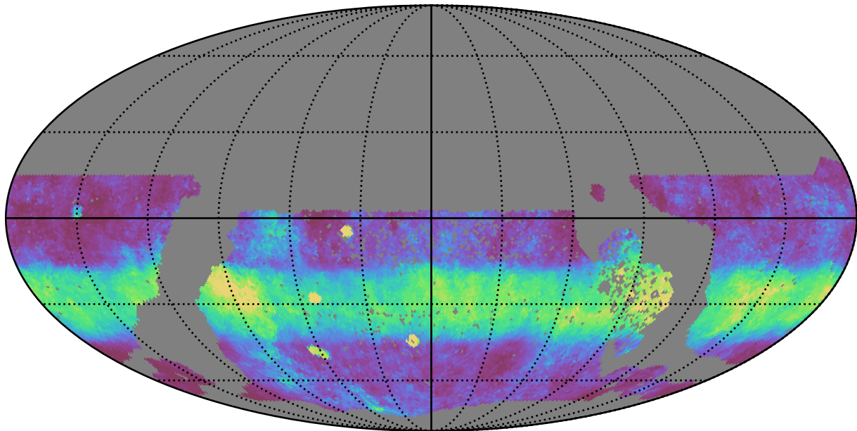
ddf_half_v3.4_10yrs WFD y band: Median normairmass
