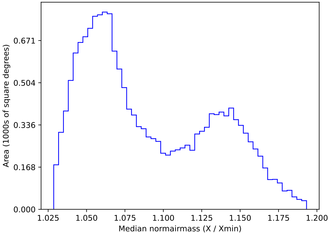
ddf_half_v3.4_10yrs WFD y band: Median normairmass
