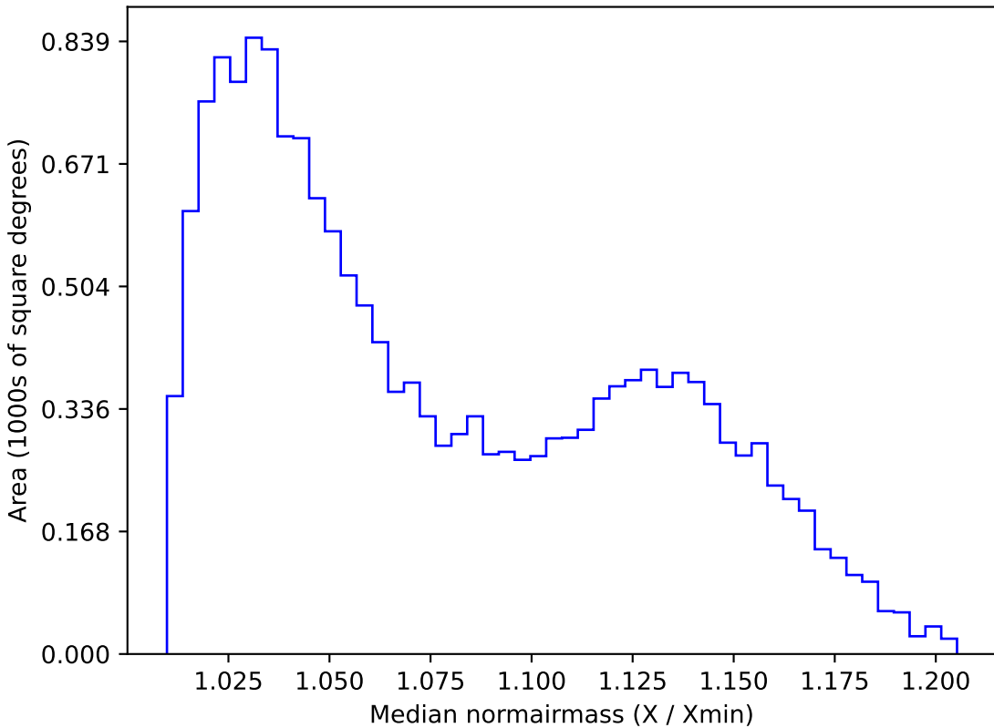
ddf_half_v3.4_10yrs WFD u band: Median normairmass
