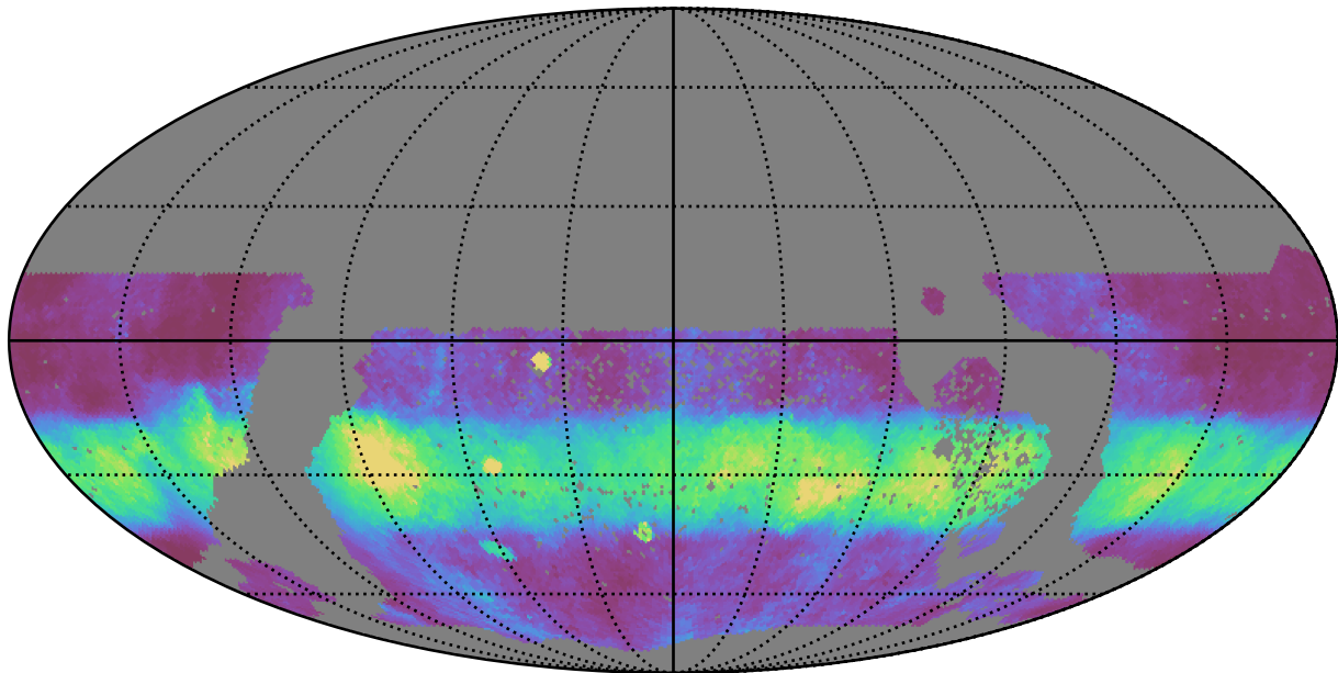
ddf_half_v3.4_10yrs WFD r band: Median normairmass
