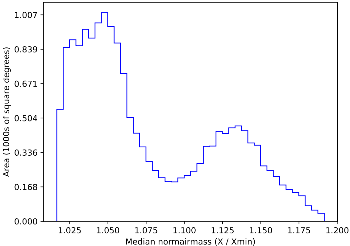
ddf_half_v3.4_10yrs WFD r band: Median normairmass
