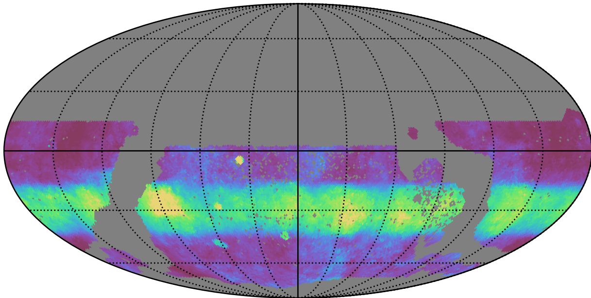
ddf_half_v3.4_10yrs WFD i band: Median normairmass
