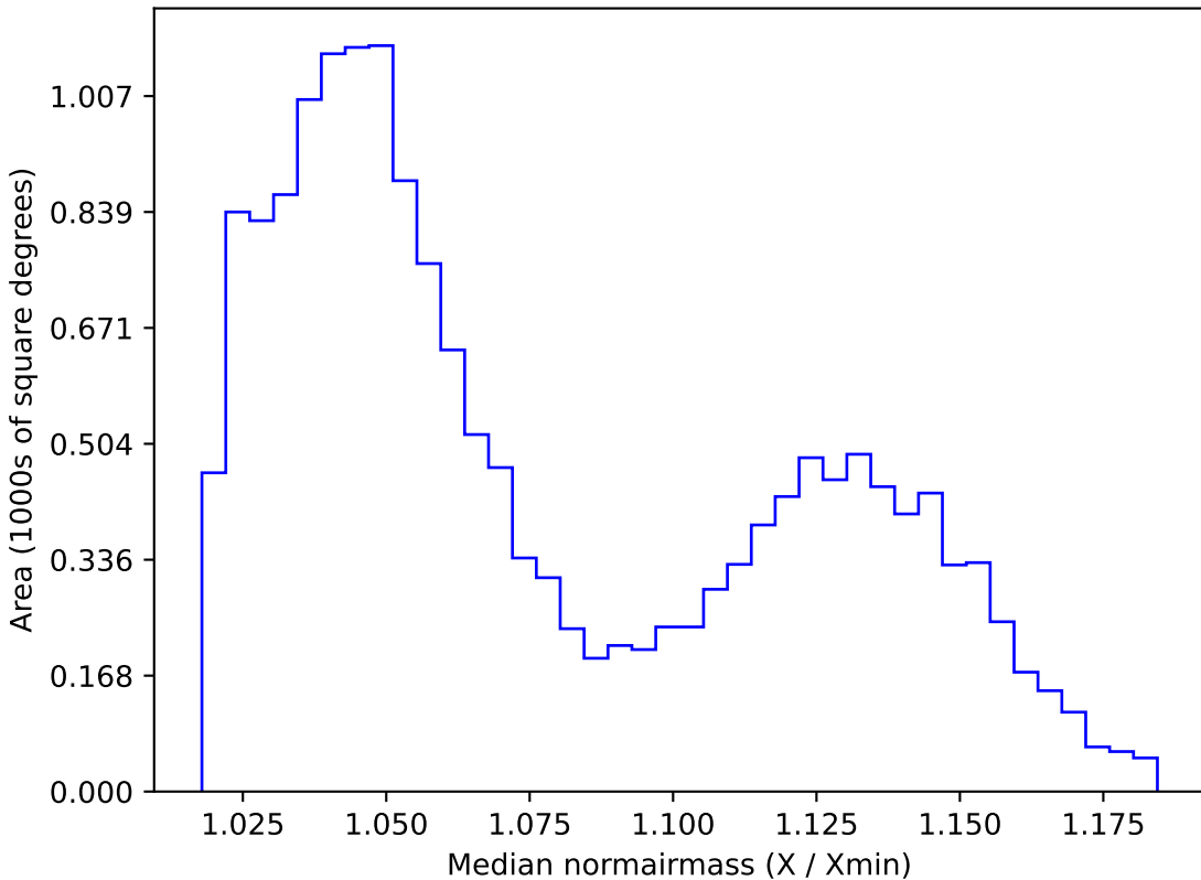
ddf_half_v3.4_10yrs WFD i band: Median normairmass
