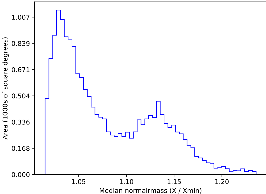
ddf_half_v3.4_10yrs WFD g band: Median normairmass
