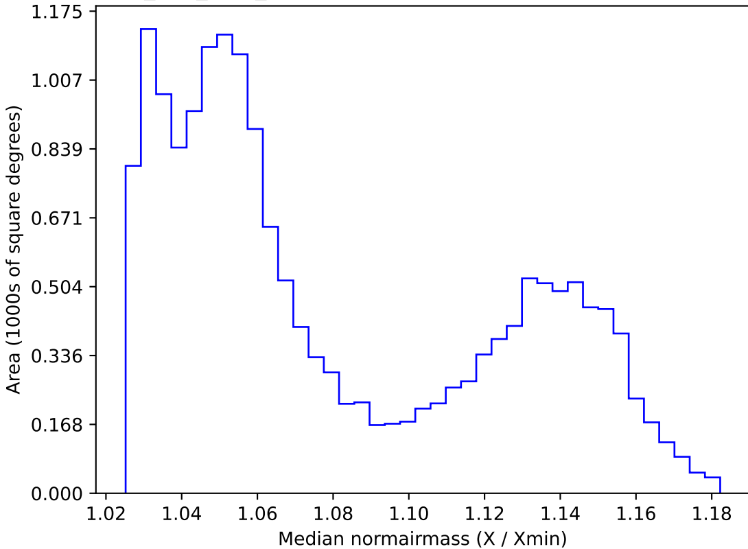
ddf_half_v3.4_10yrs WFD all bands: Median normairmass
