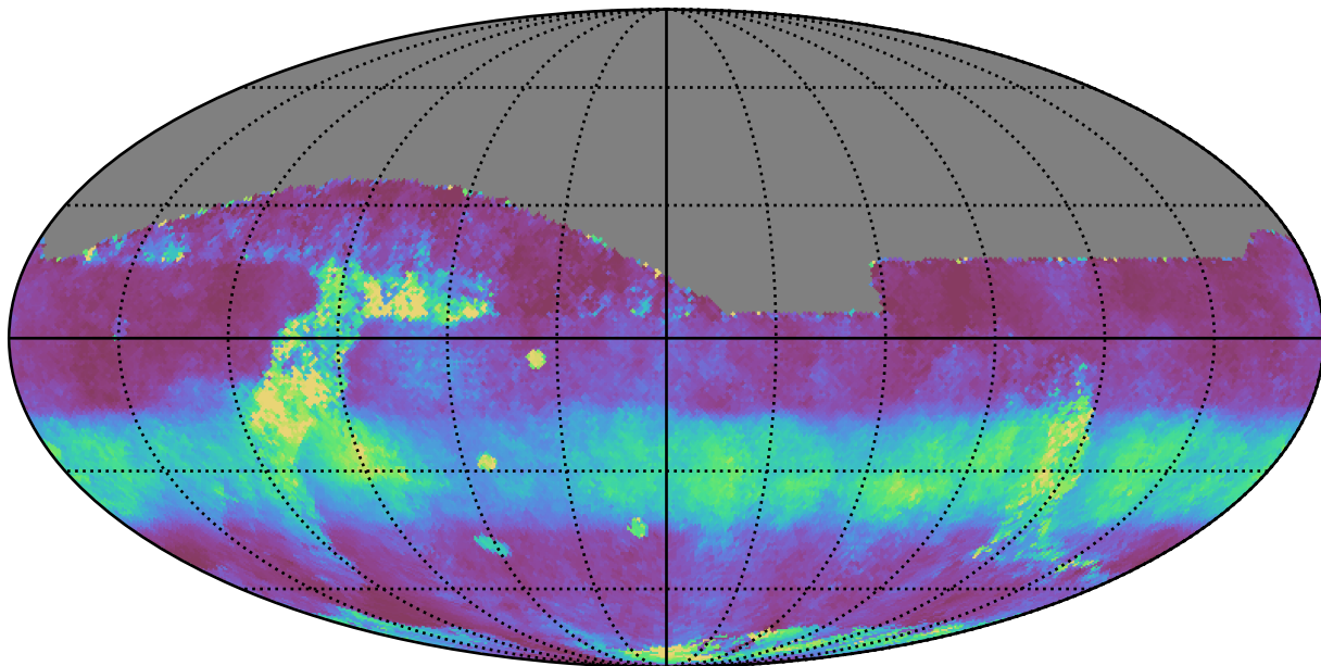
ddf_half_v3.4_10yrs All sky z band: Median normairmass
