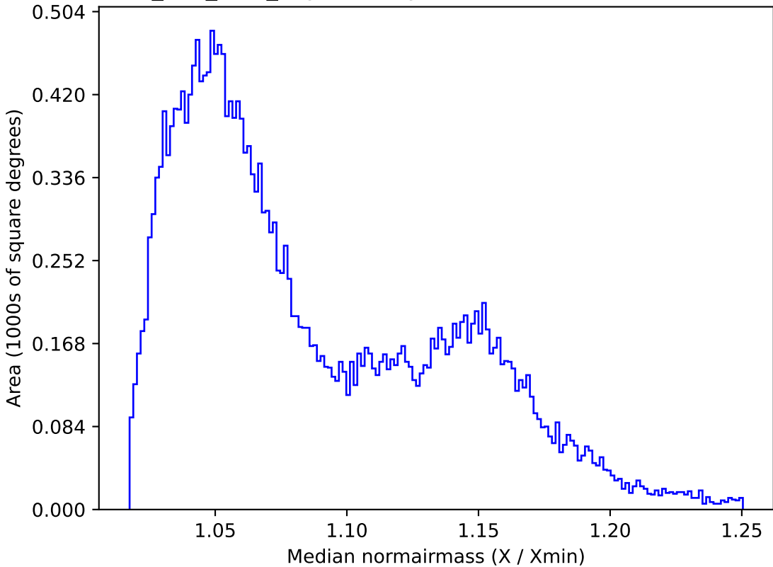
ddf_half_v3.4_10yrs All sky z band: Median normairmass
