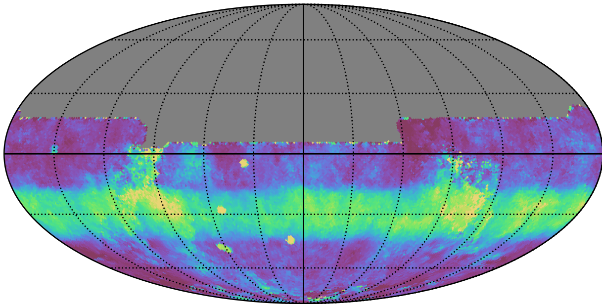
ddf_half_v3.4_10yrs All sky y band: Median normairmass
